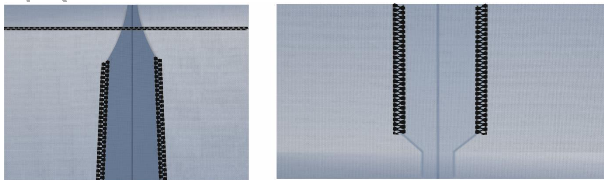
Figure: 1.59 – Trimming of corners in seams crossing another seam
