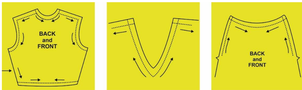
Figure: 1.67 - Direction of Stay-stitching at different areas in a garment
