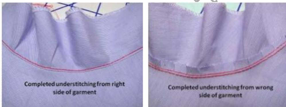
Figure: 1.65 - Under stitching
