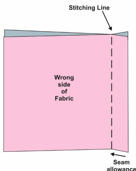
Figure: 1.40 – Plain seam
