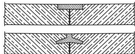
Fig. 1.24: Different forms of plug joints
