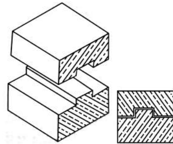
Fig. 1.22: Bed joint or tabled joint
