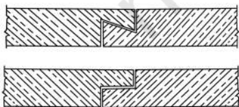
Fig. 1.21: Rebated joint
