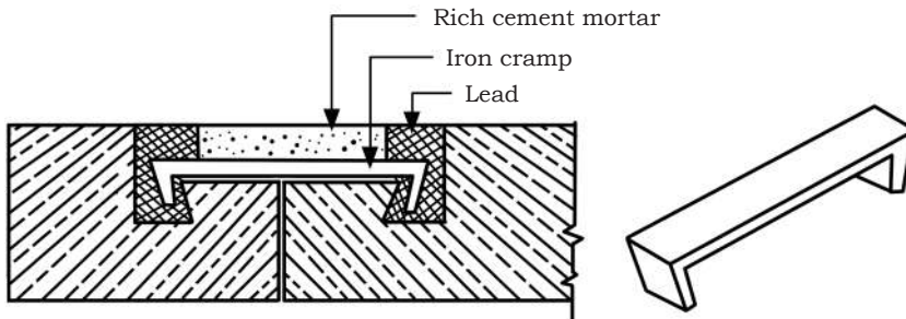
Fig. 1.26: Cramp joint
